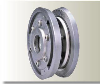
WHEEL FLANGE B05-0401 Suitable for 14"x5"x2" (55x127x50mm) grinding wheel Clamping width: 7/8"-1 1/2" (22-38mm)
