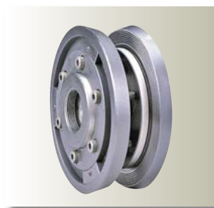
WHEEL FLANGE B05-0701 Bore size: Ø5" (127mm) Clamping width: 1.7"~2" (43-50mm)
