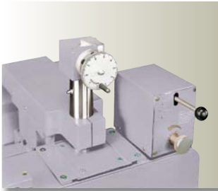
PARALLEL DRESSING ATTACHMENT (HYDRAULIC TYPE) • B13-1001 Max. OD: 14" (355mm) Mini OD: 9.3" (235mm) Max. Length: 2.4" (60mm)
